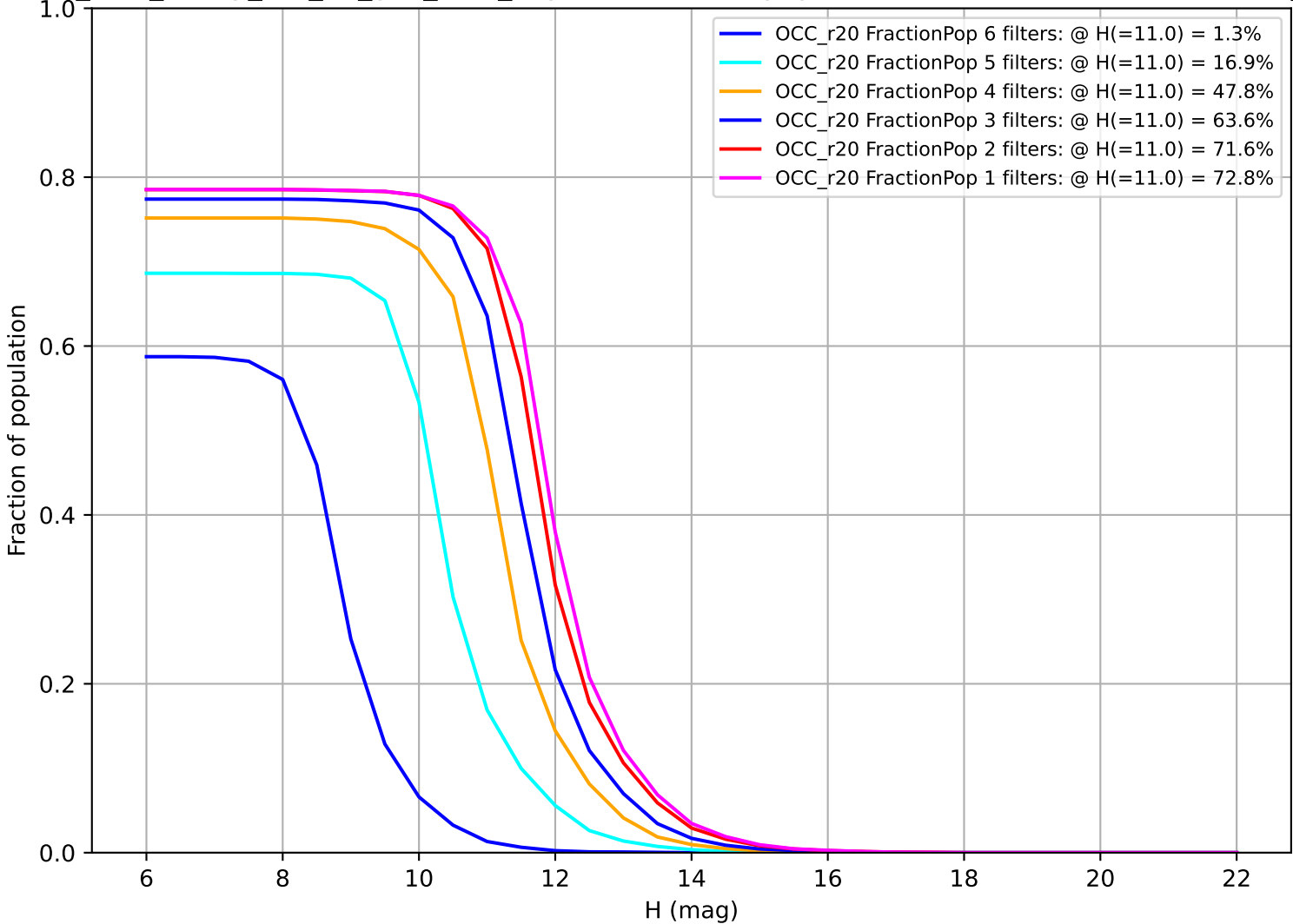
too_elab_heavy_r32_d3_griz_v3.4_10yrs: Fraction of population with colors in X filters OCC_r20
