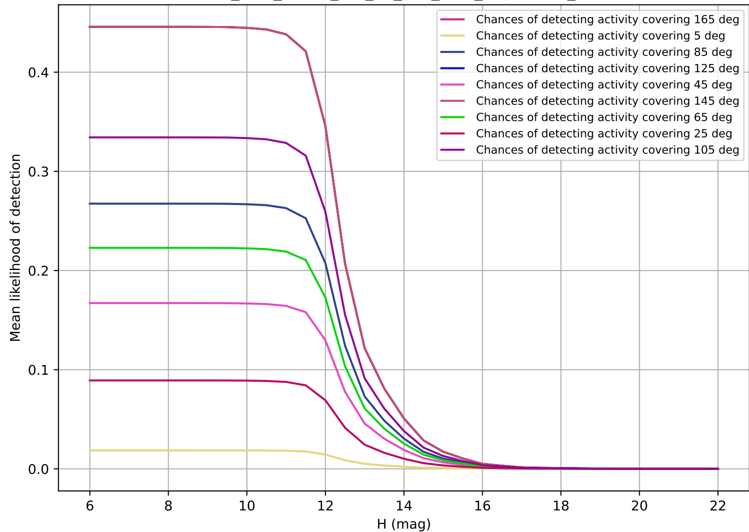
too_elab_heavy_r32_d3_griz_v3.4_10yrs OCC_r20
