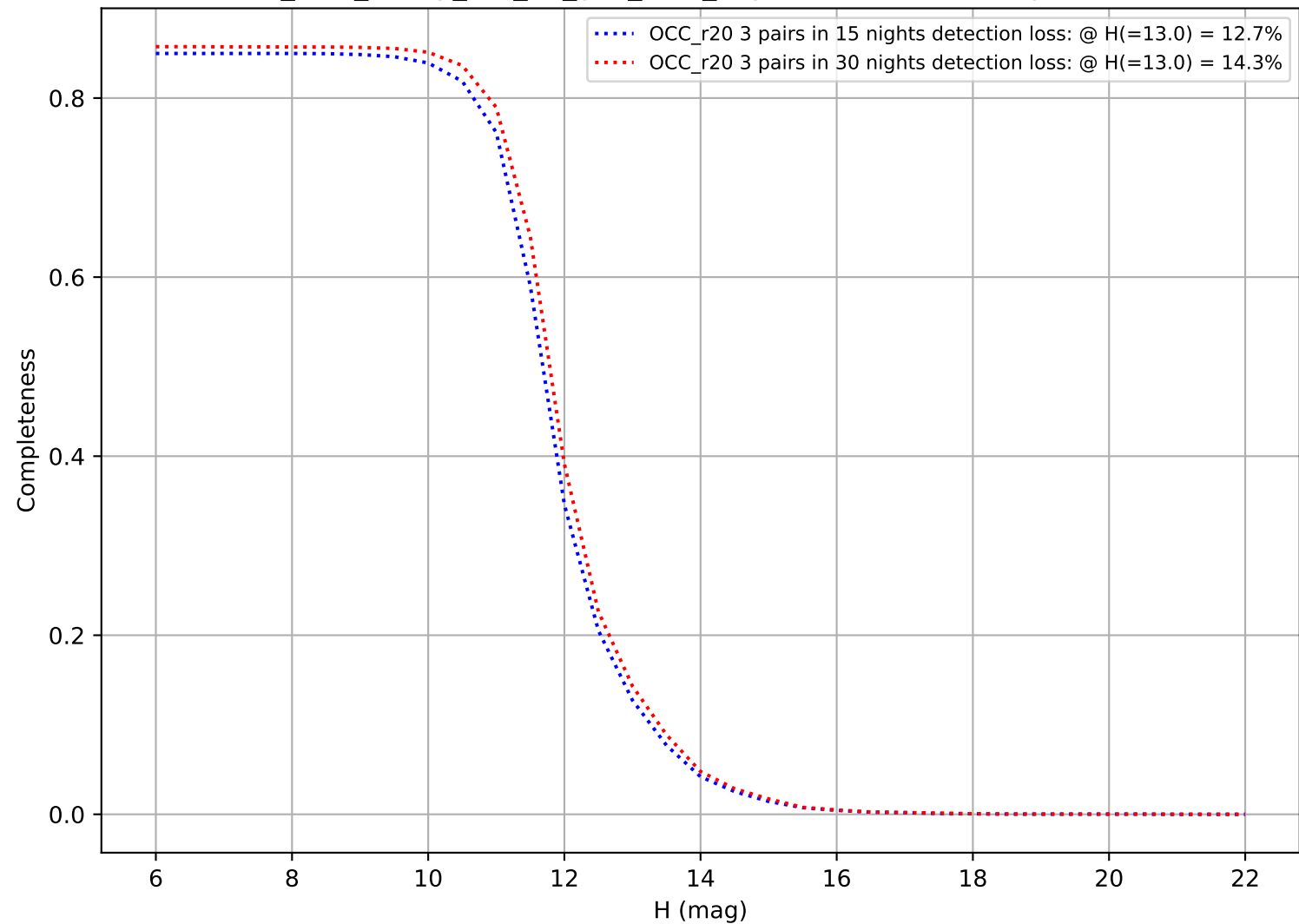
too_elab_heavy_r32_d3_griz_v3.4_10yrs: DifferentialCompleteness
