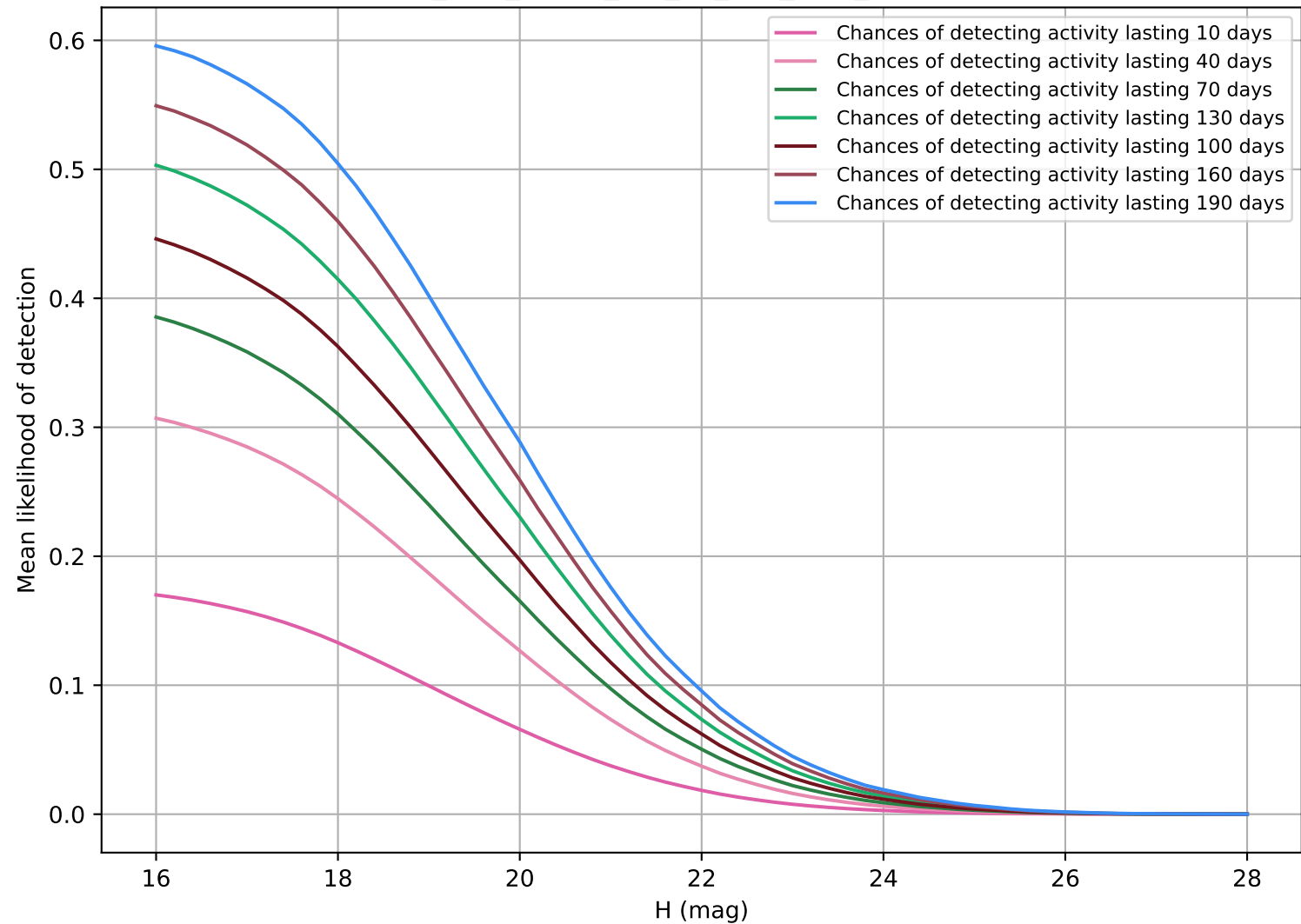
too_elab_heavy_r32_d3_griz_v3.4_10yrs NEO
