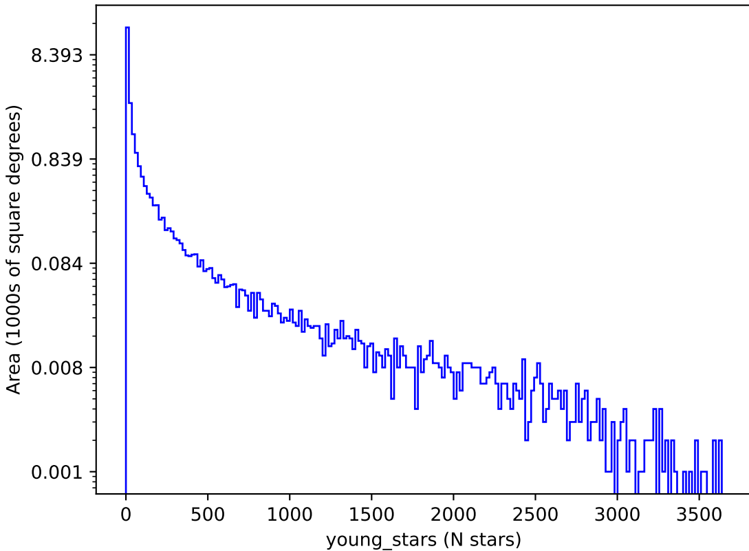
too_elab_heavy_r32_d3_griz_v3.4_10yrs : young_stars
