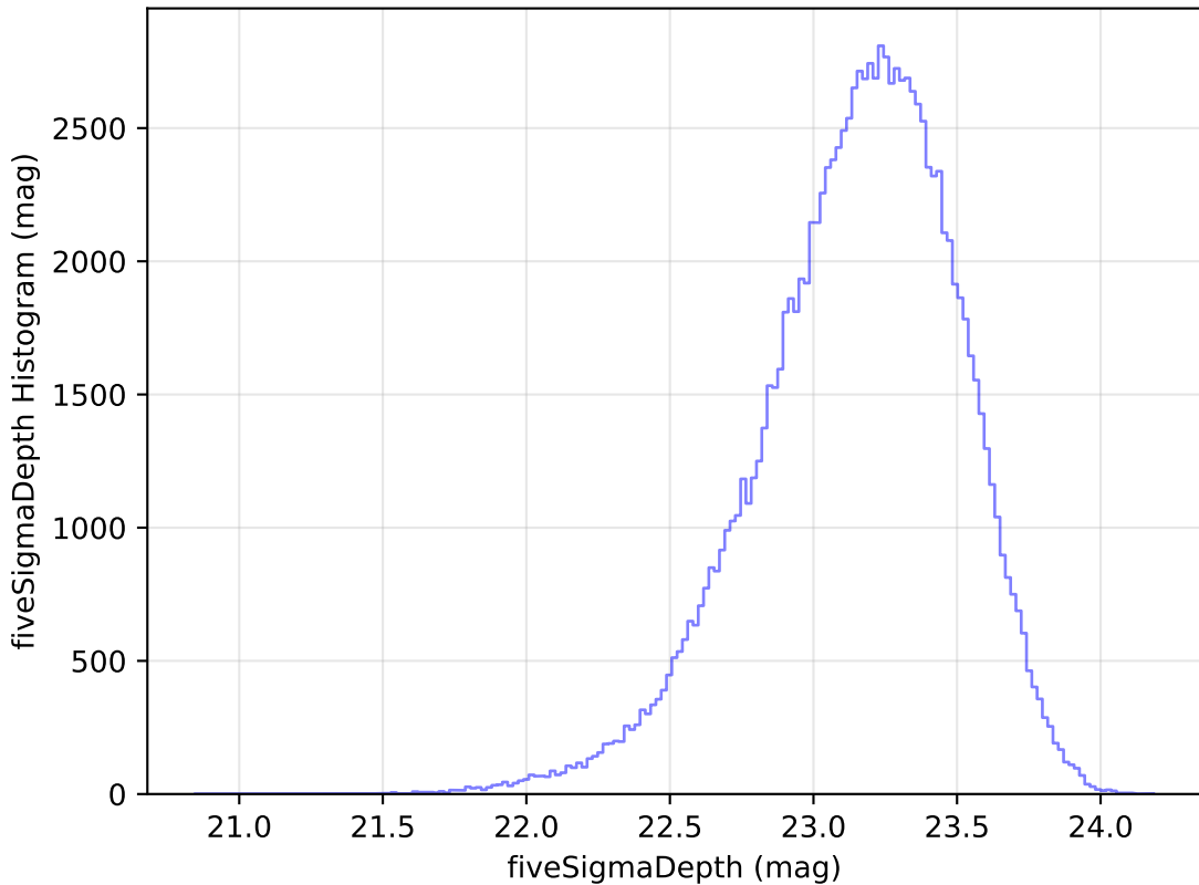
too_elab_heavy_r32_d3_griz_v3.4_10yrs u: fiveSigmaDepth Histogram
