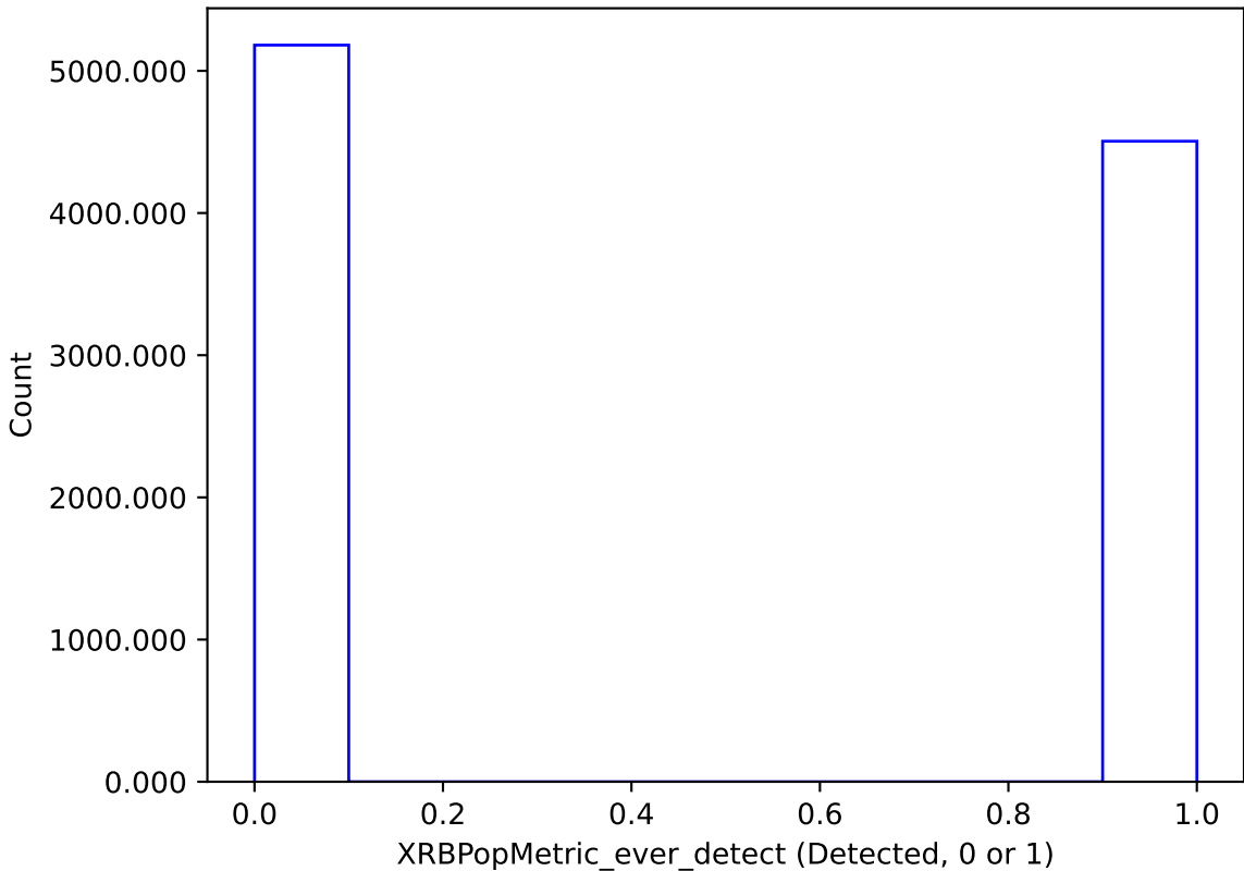
too_elab_heavy_r32_d3_griz_v3.4_10yrs : XRBPopMetric_ever_detect
