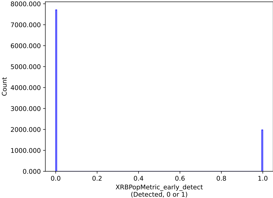
too_elab_heavy_r32_d3_griz_v3.4_10yrs : XRBPoMetric_early_detect
