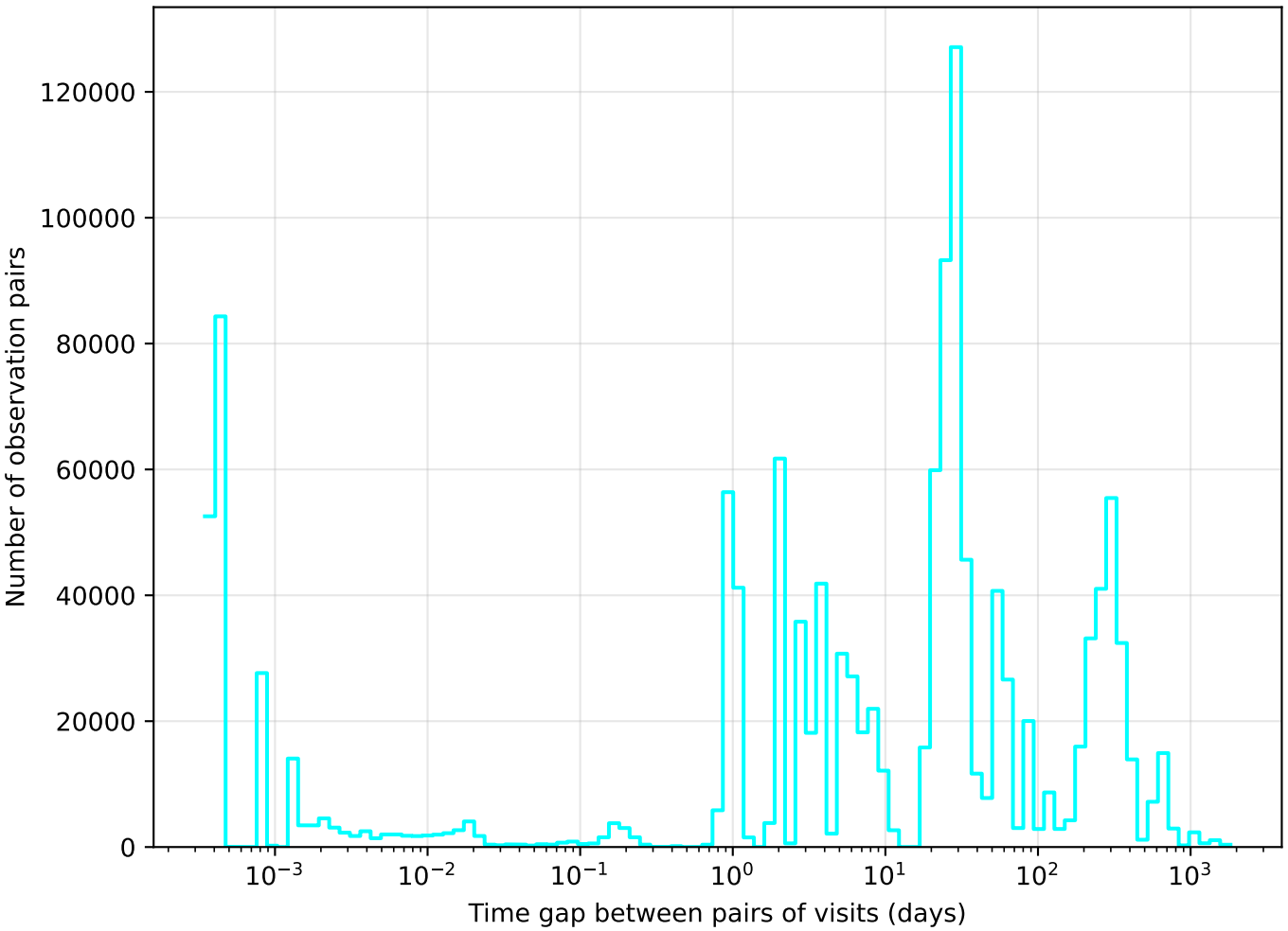
too_elab_heavy_r32_d3_griz_v3.4_10yrs u band: Tgaps observationStartMJD
