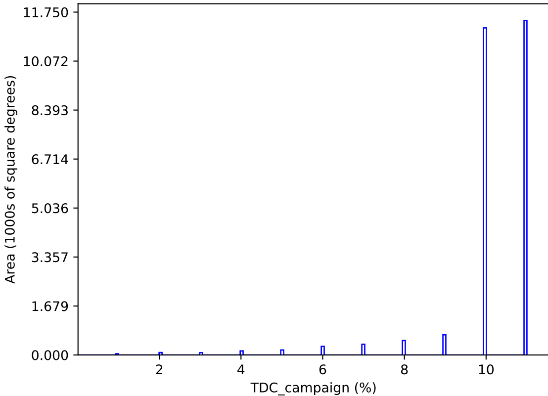
too_elab_heavy_r32_d3_griz_v3.4_10yrs : TDC_campaign
