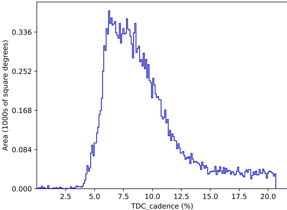
too_elab_heavy_r32_d3_griz_v3.4_10yrs : TDC_cadence
