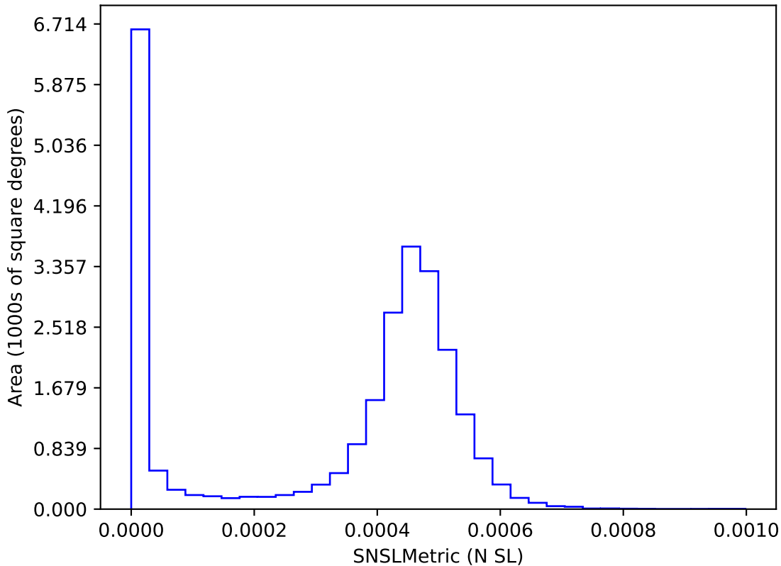
too_elab_heavy_r32_d3_griz_v3.4_10yrs : SNSLMetric
