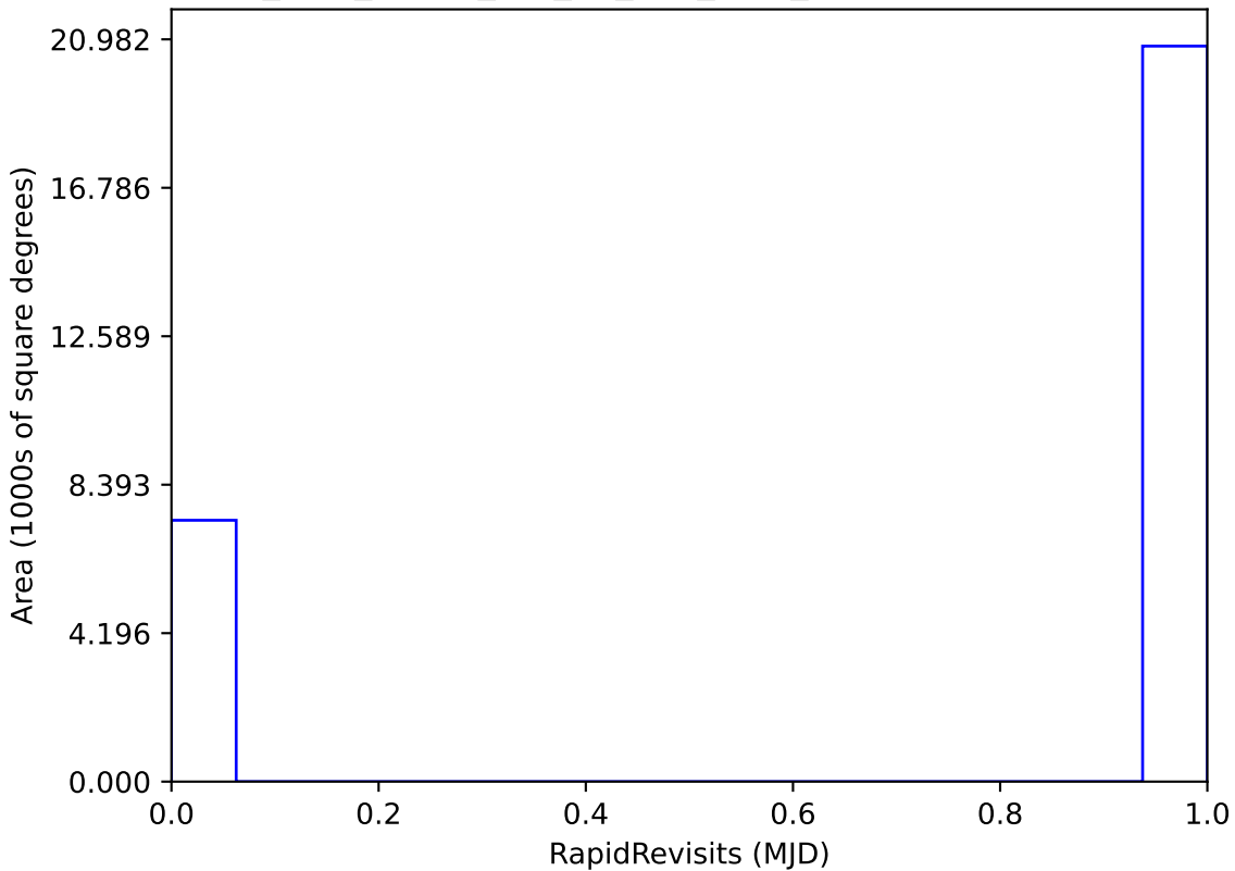
too_elab_heavy_r32_d3_griz_v3.4_10yrs : RapidRevisits
