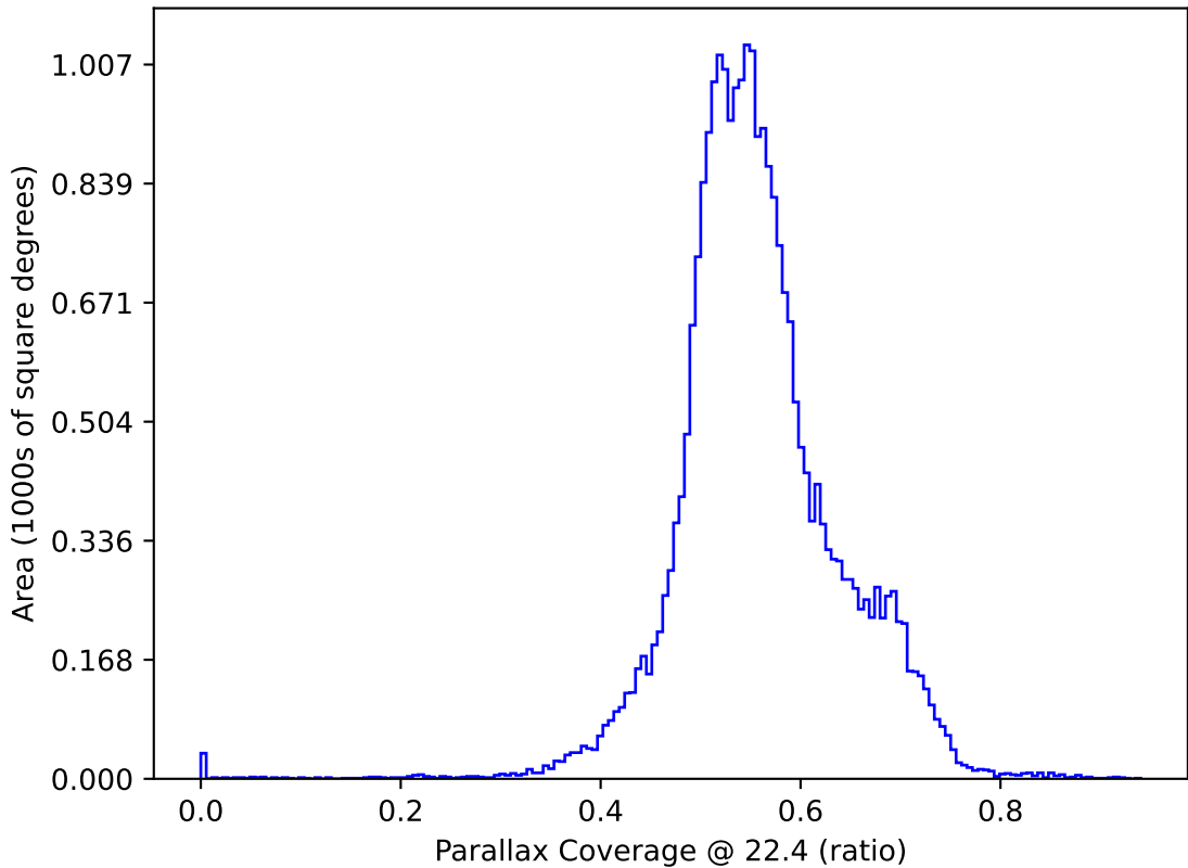
too_elab_heavy_r32_d3_griz_v3.4_10yrs : Parallax Coverage @ 22.4
