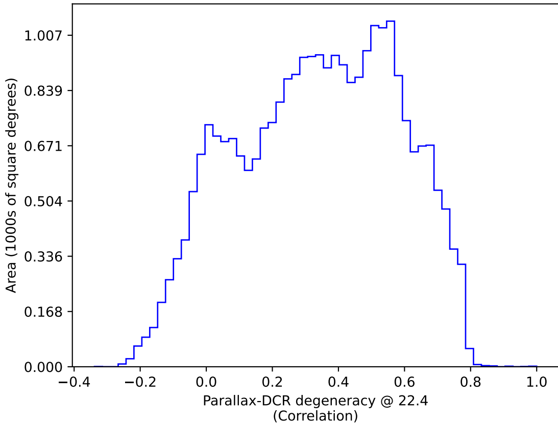
too_elab_heavy_r32_d3_griz_v3.4_10yrs : Parallax-DCR degeneracy @ 22.4
