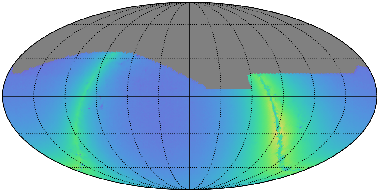
too_elab_heavy_r32_d3_griz_v3.4_10yrs i: Nstars_no_crowding
