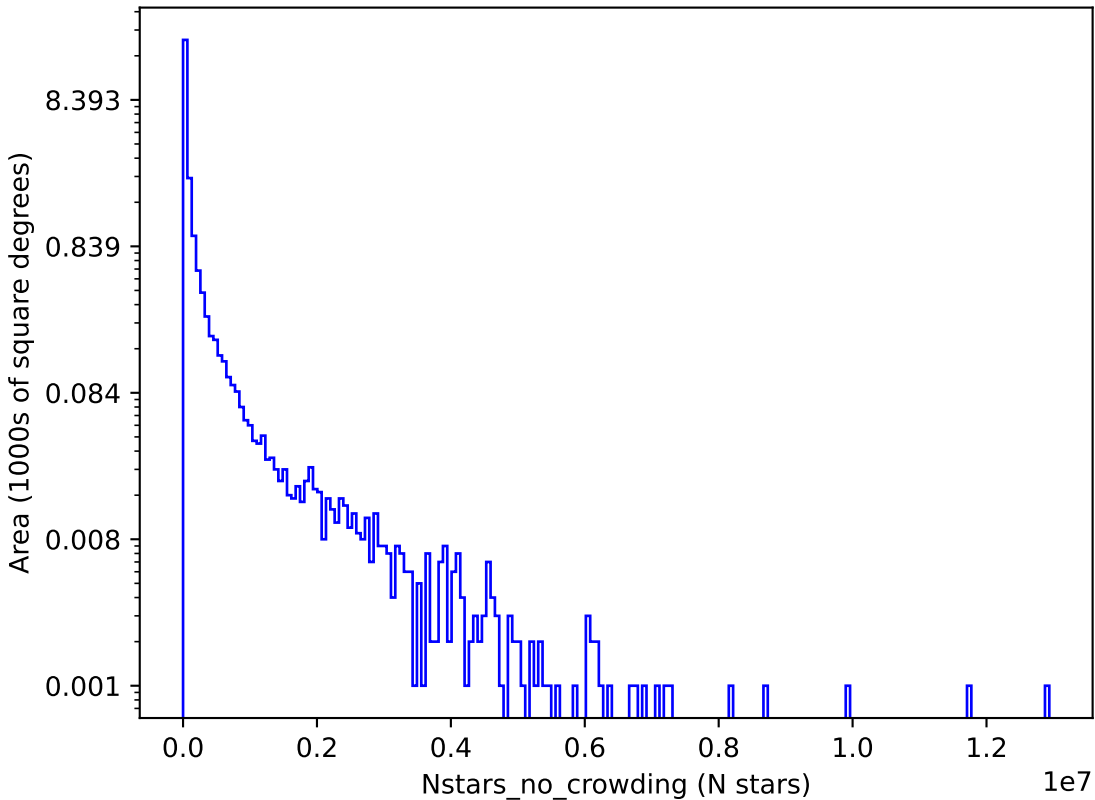
too_elab_heavy_r32_d3_griz_v3.4_10yrs g: Nstars_no_crowding
