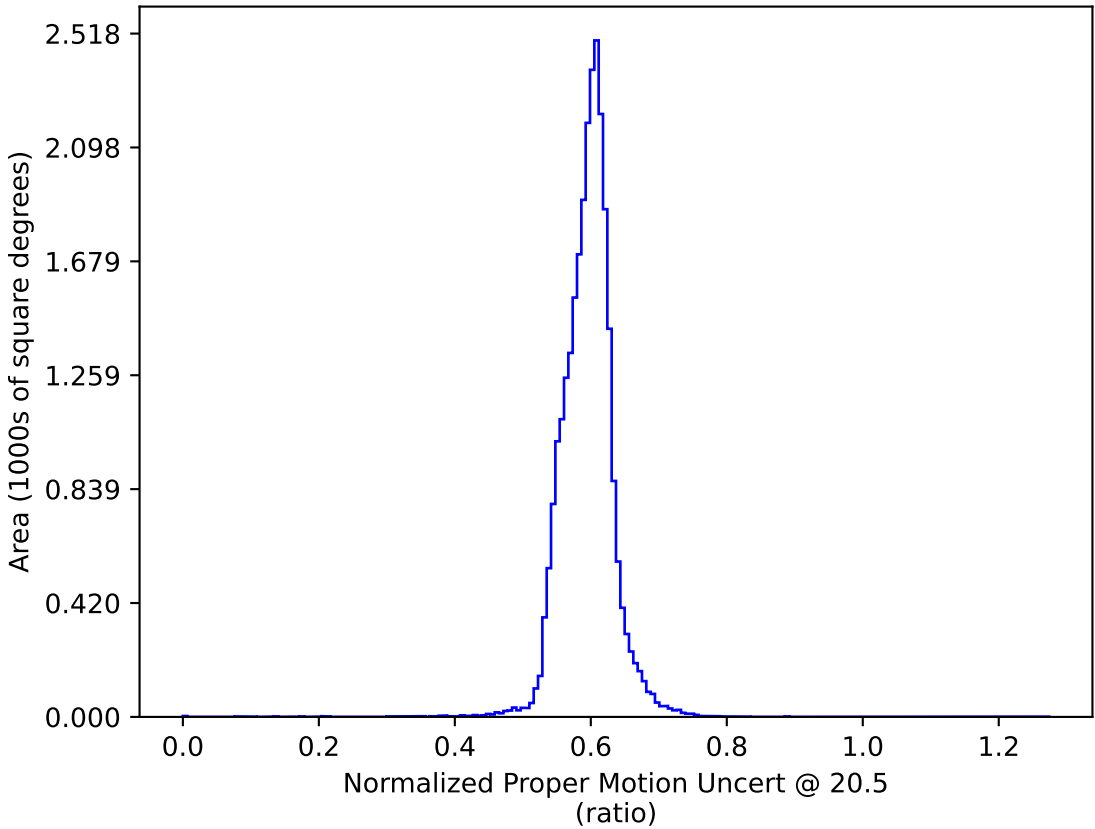
too_elab_heavy_r32_d3_griz_v3.4_10yrs : Normalized Proper Motion Uncert @ 20.5
