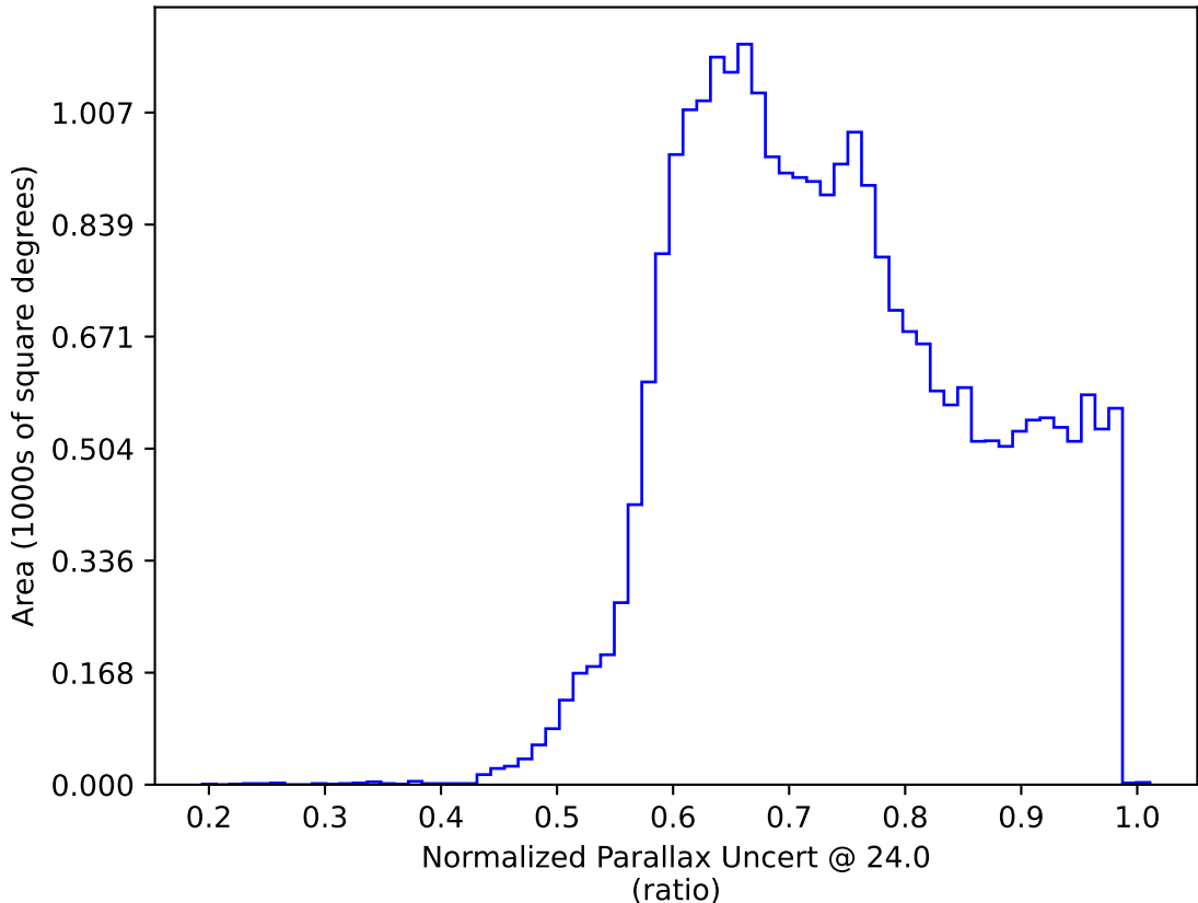
too_elab_heavy_r32_d3_griz_v3.4_10yrs : Normalized Parallax Uncert @ 24.0
