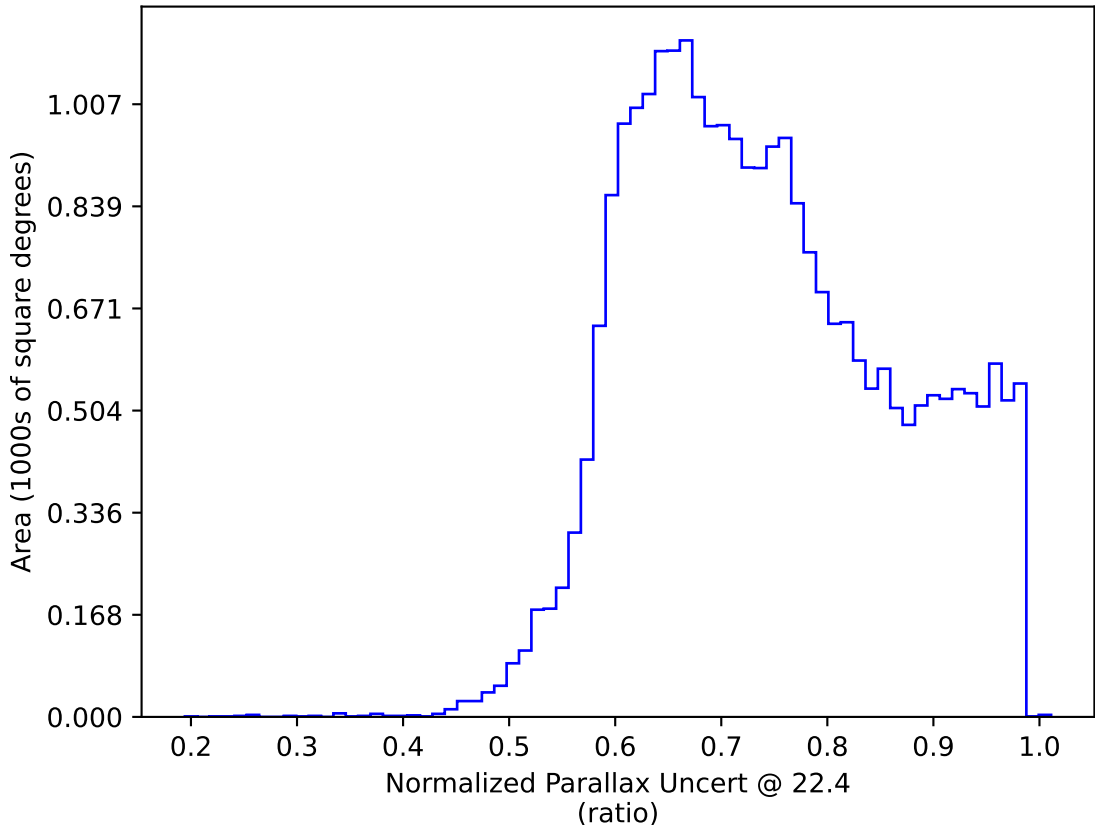
too_elab_heavy_r32_d3_griz_v3.4_10yrs : Normalized Parallax Uncert @ 22.4
