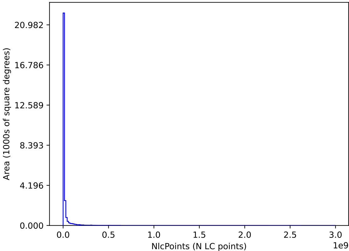
too_elab_heavy_r32_d3_griz_v3.4_10yrs : NlcPoints
