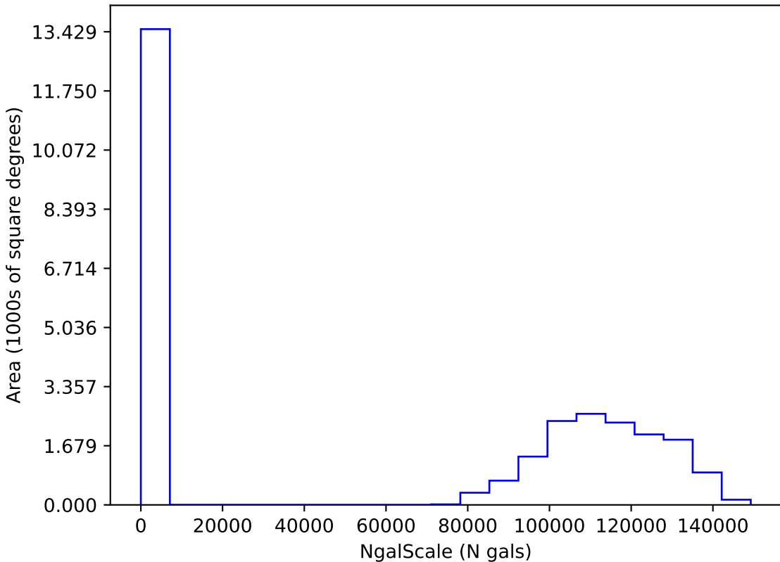
too_elab_heavy_r32_d3_griz_v3.4_10yrs i: NgalScale
