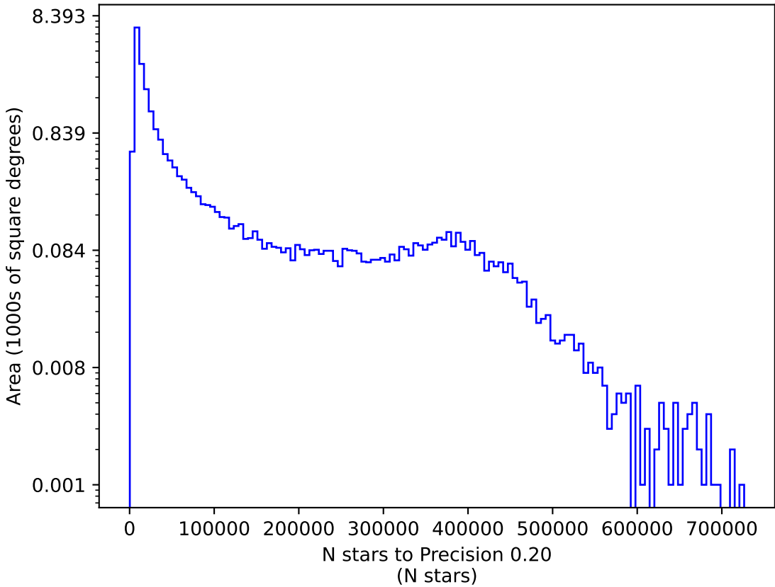
too_elab_heavy_r32_d3_griz_v3.4_10yrs y: N stars to Precision 0.20
