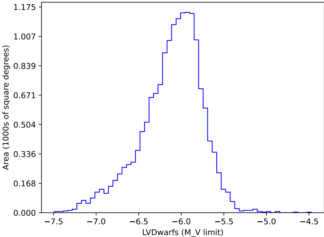
too_elab_heavy_r32_d3_griz_v3.4_10yrs gi: LVDwarfs
