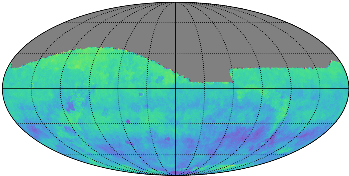
too_elab_heavy_r32_d3_griz_v3.4_10yrs i: Kuiper rotSkyPos
