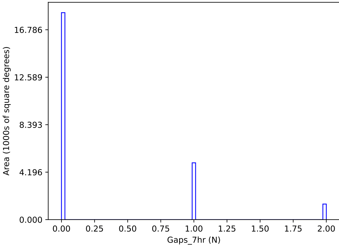
too_elab_heavy_r32_d3_griz_v3.4_10yrs y band: Gaps_7hr
