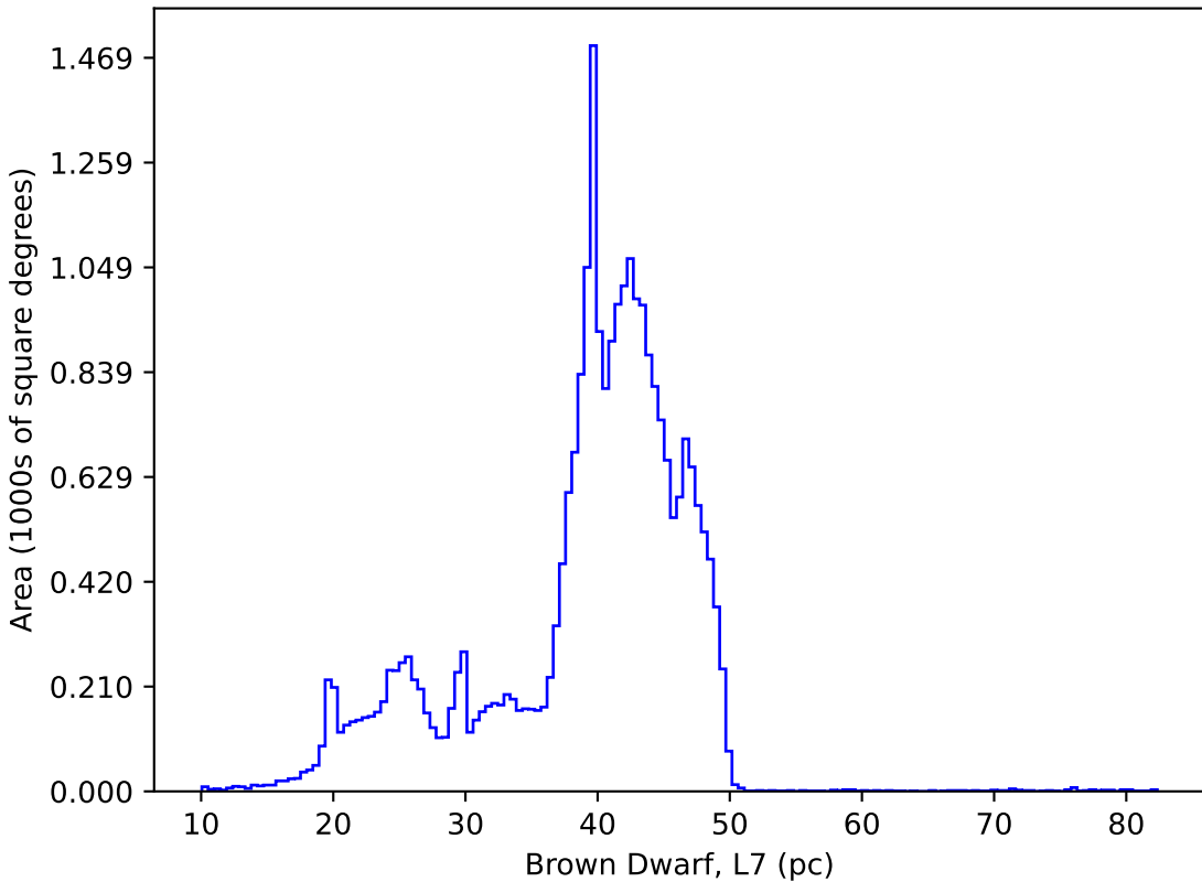
too_elab_heavy_r32_d3_griz_v3.4_10yrs : Brown Dwarf, L7
