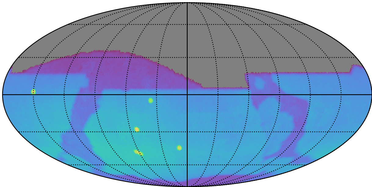
too_elab_heavy_r32_d3_griz_v3.4_10yrs : Brown Dwarf, L4
