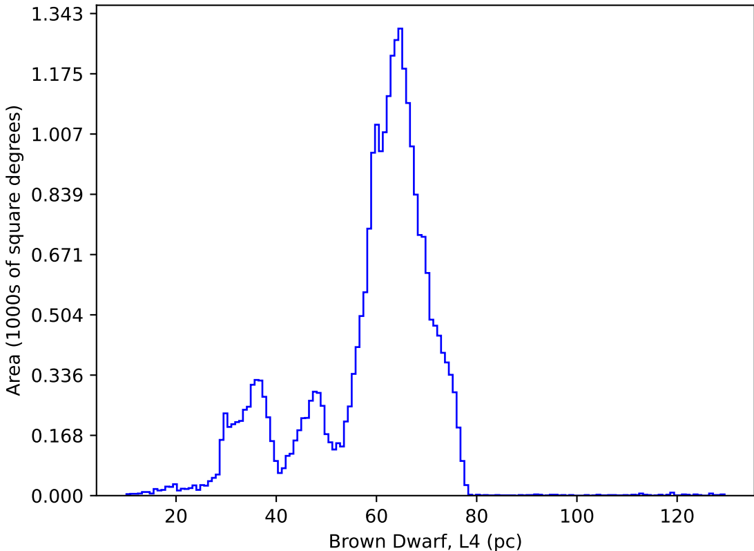
too_elab_heavy_r32_d3_griz_v3.4_10yrs : Brown Dwarf, L4
