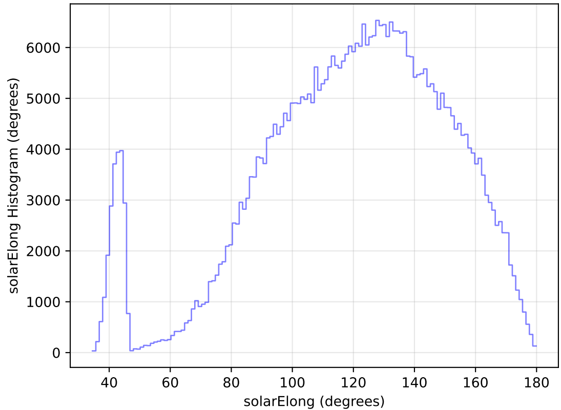
too_elab_heavy_r32_d3_griz_v3.4_10yrs WFD z band: solarElong Histogram
