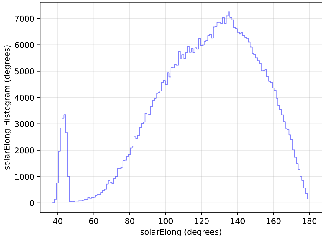
too_elab_heavy_r32_d3_griz_v3.4_10yrs WFD r band: solarElong Histogram
