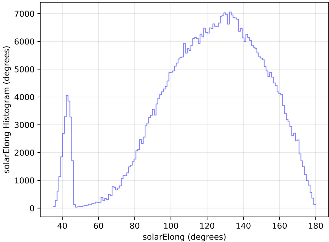
too_elab_heavy_r32_d3_griz_v3.4_10yrs WFD i band: solarElong Histogram
