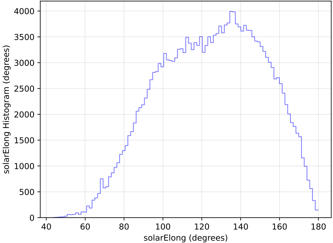
too_elab_heavy_r32_d3_griz_v3.4_10yrs WFD g band: solarElong Histogram
