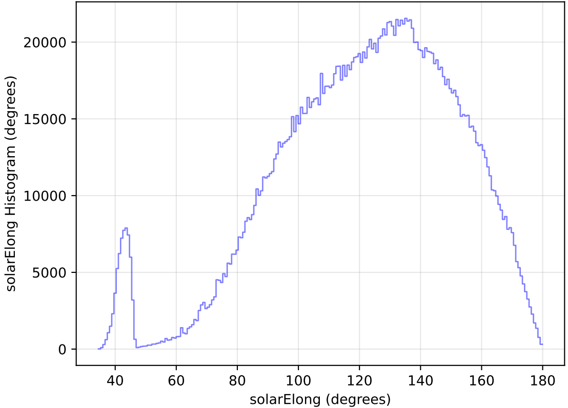
too_elab_heavy_r32_d3_griz_v3.4_10yrs WFD all bands: solarElong Histogram
