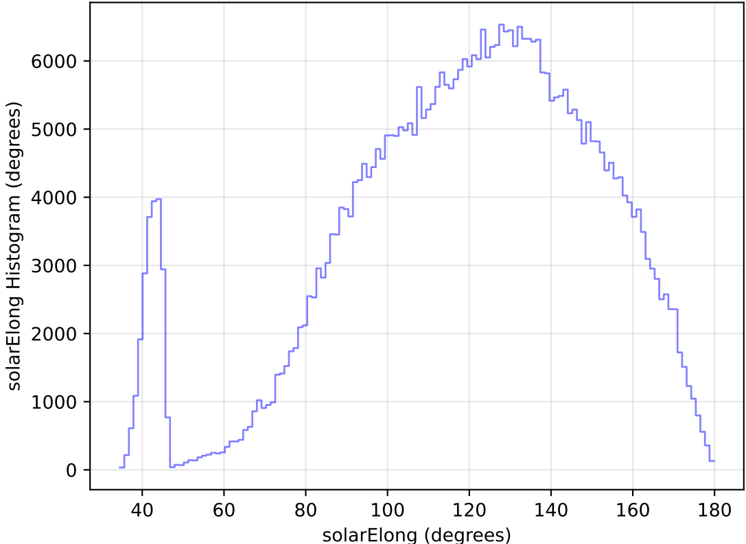
too_elab_heavy_r32_d3_griz_v3.4_10yrs All sky z band: solarElong Histogram
