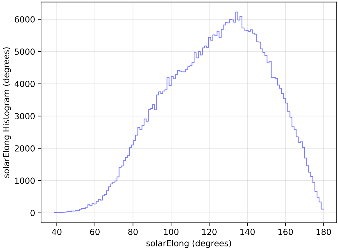
too_elab_heavy_r32_d3_griz_v3.4_10yrs All sky y band: solarElong Histogram
