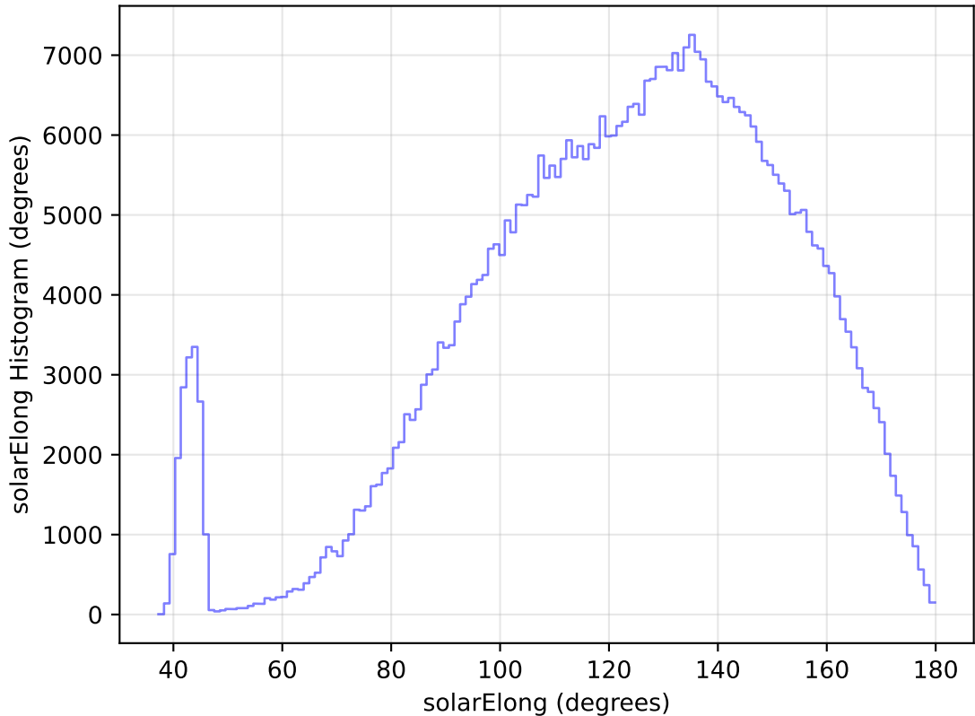
too_elab_heavy_r32_d3_griz_v3.4_10yrs All sky r band: solarElong Histogram
