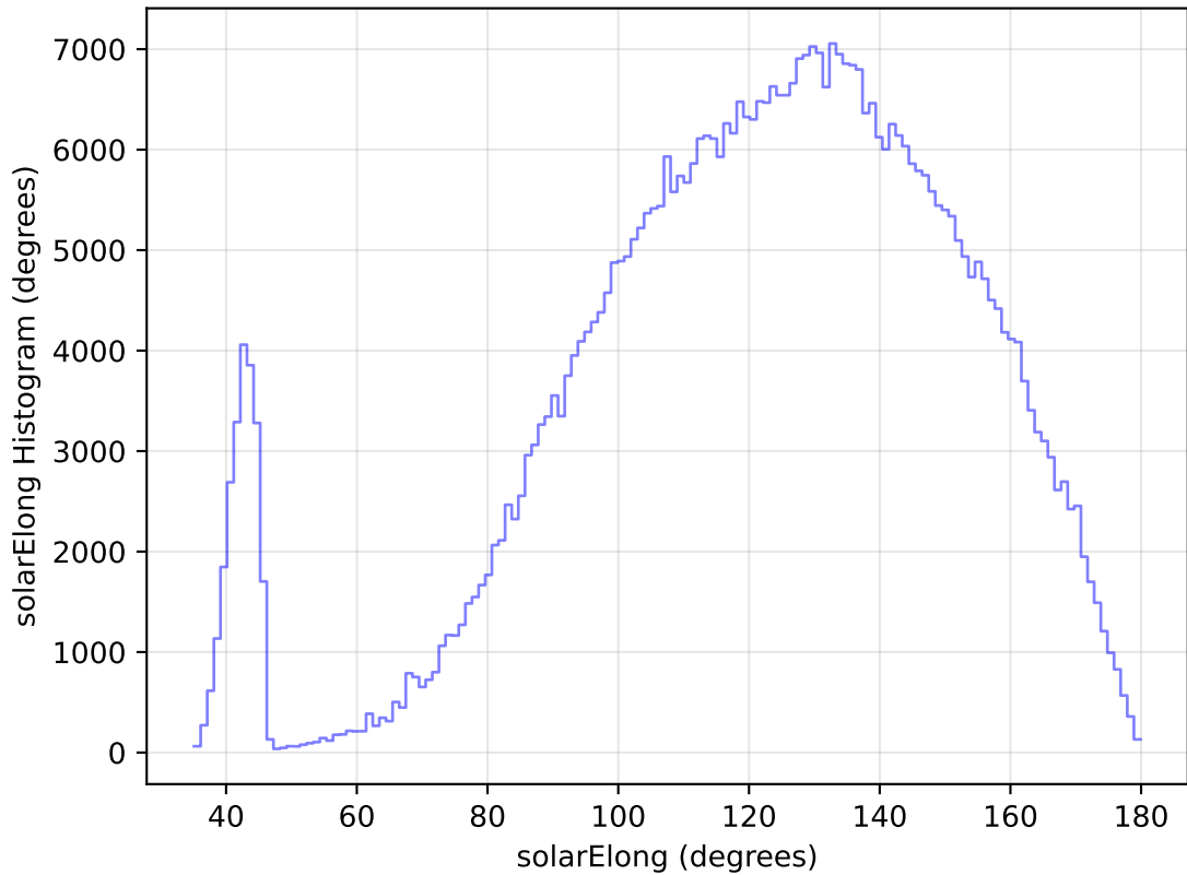
too_elab_heavy_r32_d3_griz_v3.4_10yrs All sky i band: solarElong Histogram
