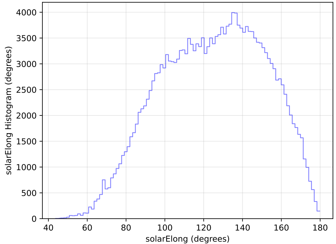
too_elab_heavy_r32_d3_griz_v3.4_10yrs All sky g band: solarElong Histogram
