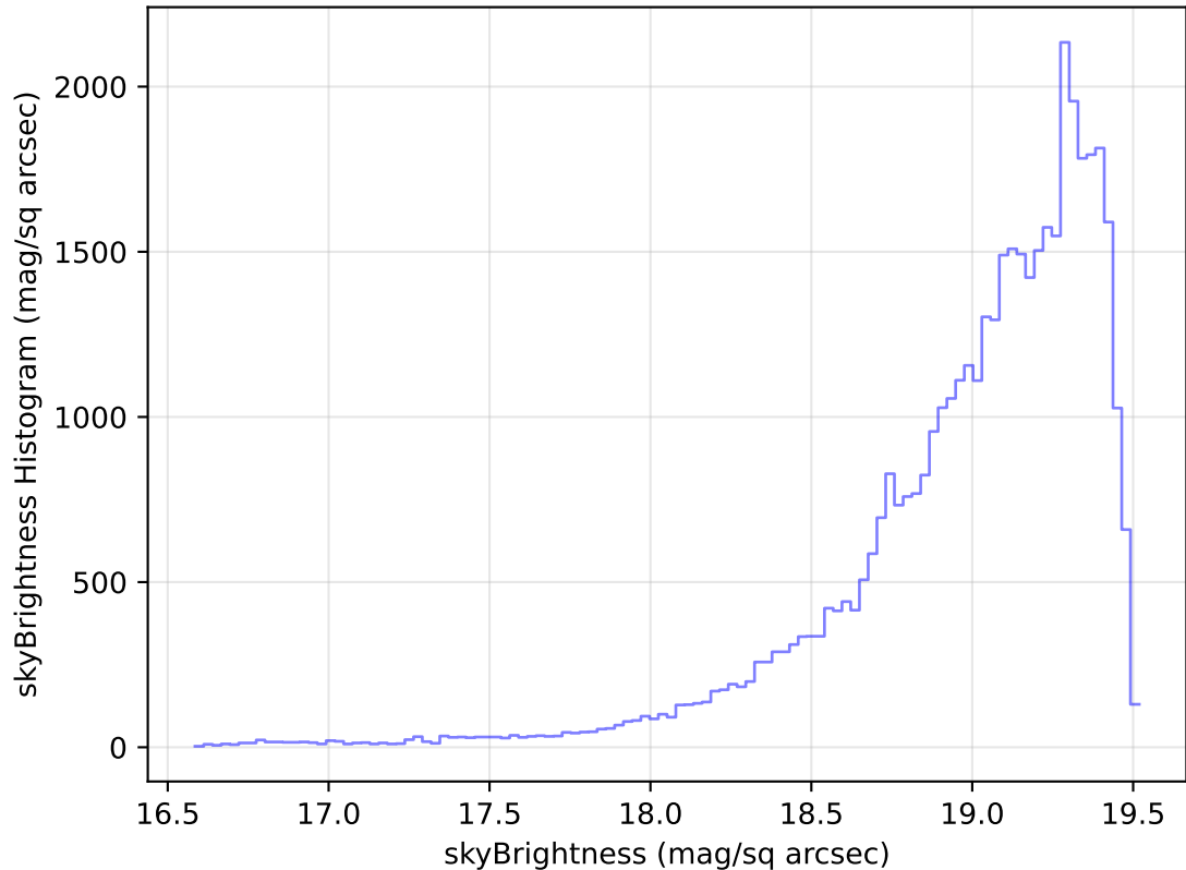
too_elab_heavy_r32_d3_griz_v3.4_10yrs Yr 1 z band: skyBrightness Histogram
