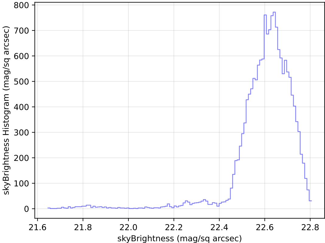
too_elab_heavy_r32_d3_griz_v3.4_10yrs Yr 1 u band: skyBrightness Histogram
