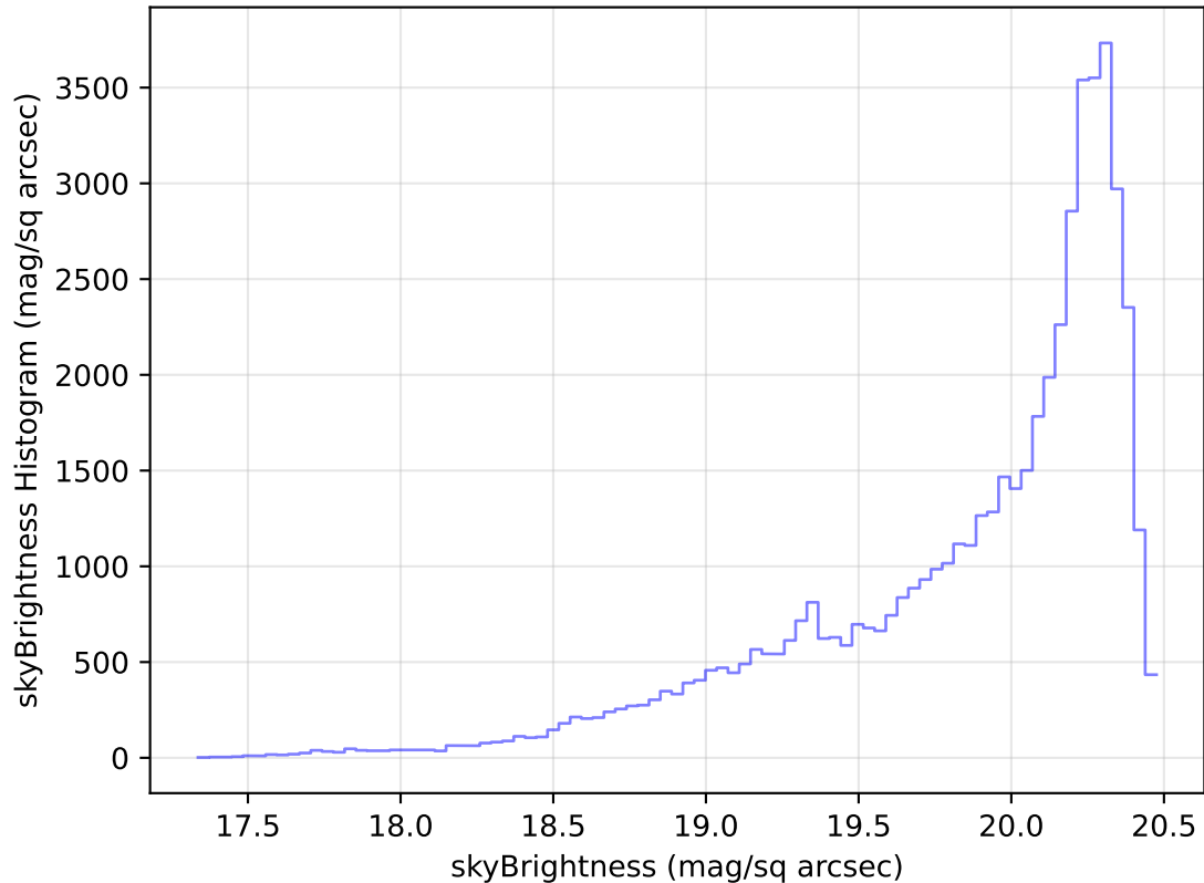
too_elab_heavy_r32_d3_griz_v3.4_10yrs Yr 1 i band: skyBrightness Histogram
