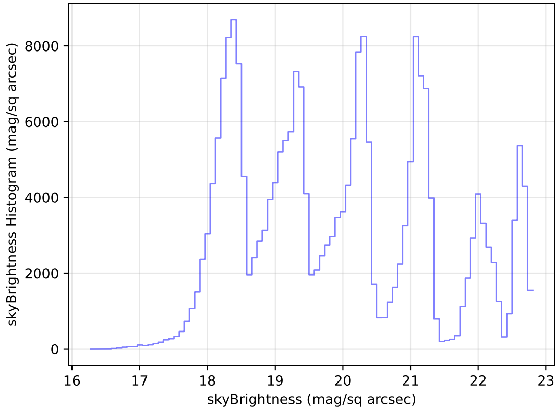
too_elab_heavy_r32_d3_griz_v3.4_10yrs Yr 1 all bands: skyBrightness Histogram
