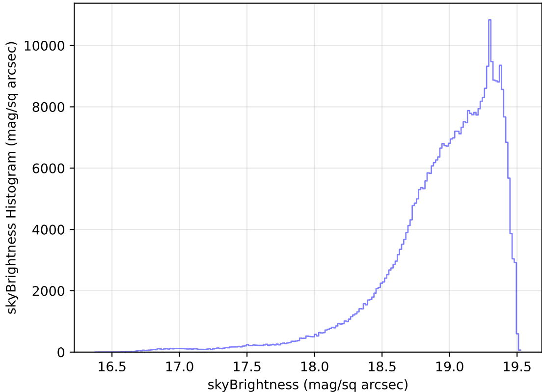
too_elab_heavy_r32_d3_griz_v3.4_10yrs WFD z band: skyBrightness Histogram
