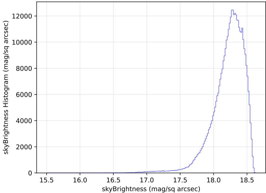
too_elab_heavy_r32_d3_griz_v3.4_10yrs WFD y band: skyBrightness Histogram
