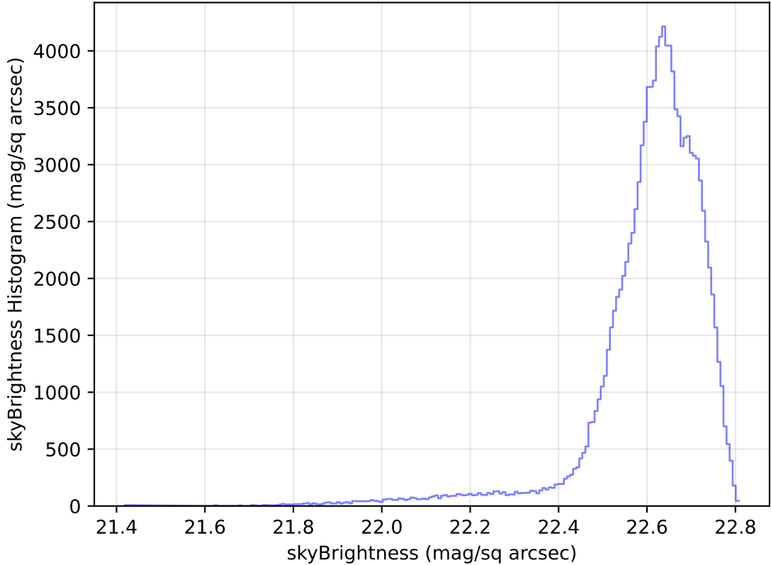
too_elab_heavy_r32_d3_griz_v3.4_10yrs WFD u band: skyBrightness Histogram
