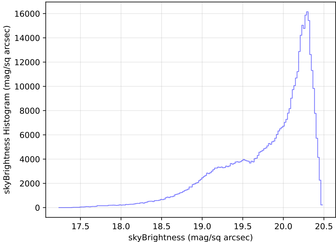
too_elab_heavy_r32_d3_griz_v3.4_10yrs WFD i band: skyBrightness Histogram
