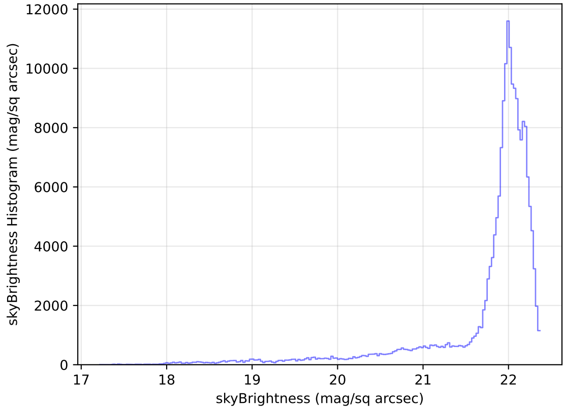
too_elab_heavy_r32_d3_griz_v3.4_10yrs WFD g band: skyBrightness Histogram
