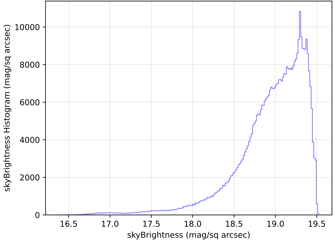
too_elab_heavy_r32_d3_griz_v3.4_10yrs All sky z band: skyBrightness Histogram
