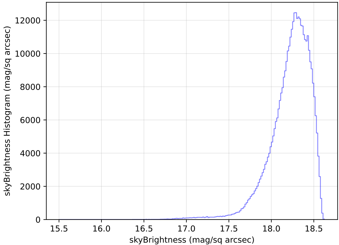
too_elab_heavy_r32_d3_griz_v3.4_10yrs All sky y band: skyBrightness Histogram
